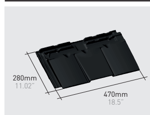
Q96*K | Visum3 ventilation roof tile klinker
