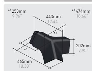
Q94*K | Pyramid triple ridge klinker
